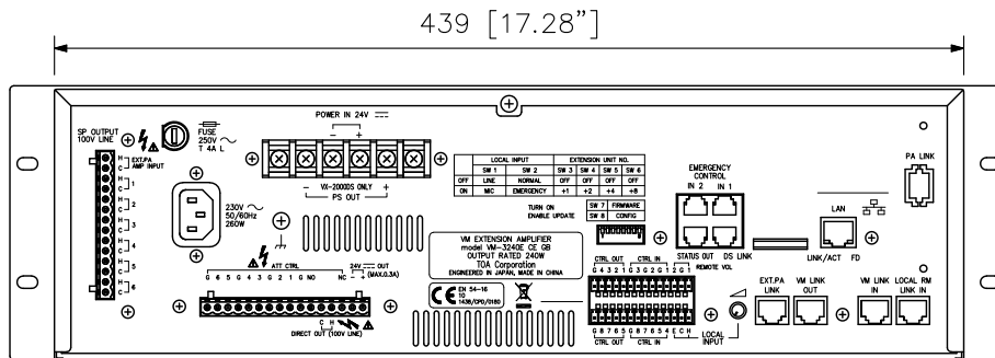
Rear View
