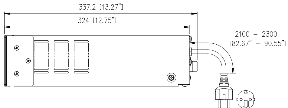
Right View
