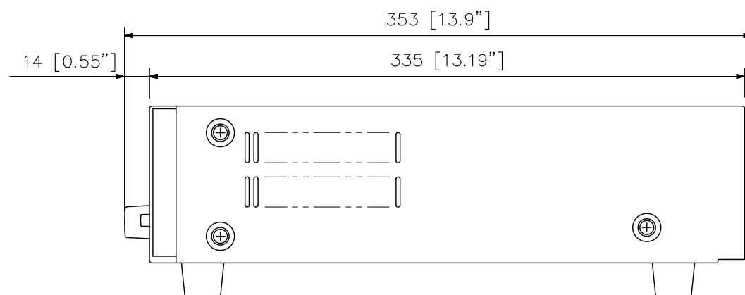
Side View
