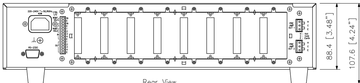
Rear View
