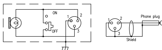
Circuit Diagram
