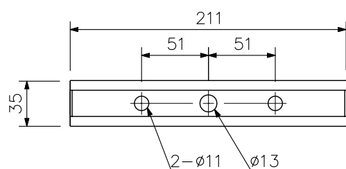
Dimensional Diagram
