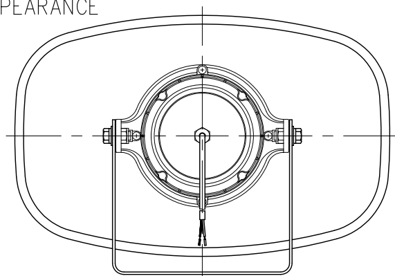
Rear View
