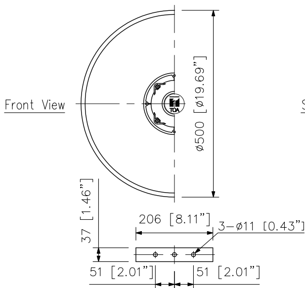
Bracket dimensional diagram
