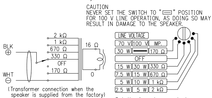
Wiring diagram
