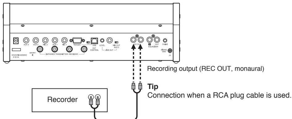
Central unit TS-920RC (Rear panel)
