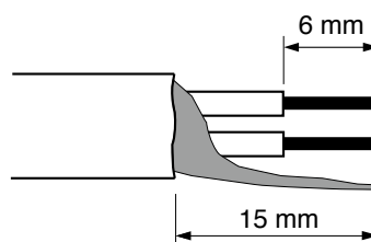
Shielded cable
