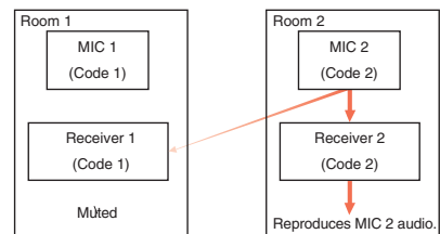
Figure c. If different codes are set in Area 1 and Area 2, mistake reception will not occur even if power to the microphone for either area is turned off. (Since microphones in both areas differ in code, audio is muted.)
