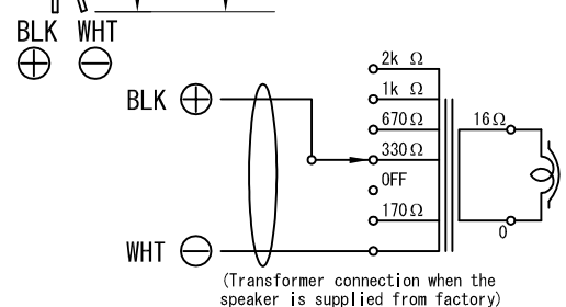
Wiring diagram
