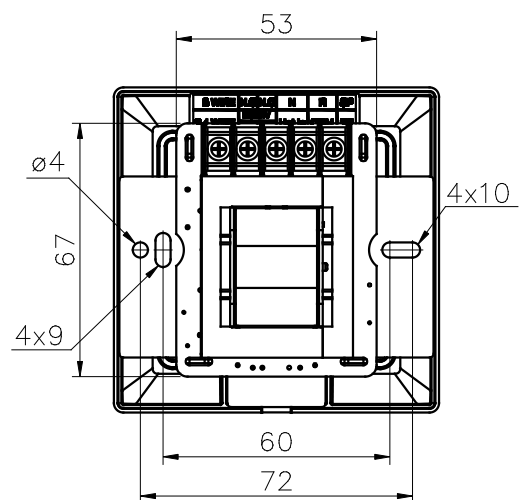
Rear View
