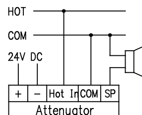
4 - WIRE CONNECTION
