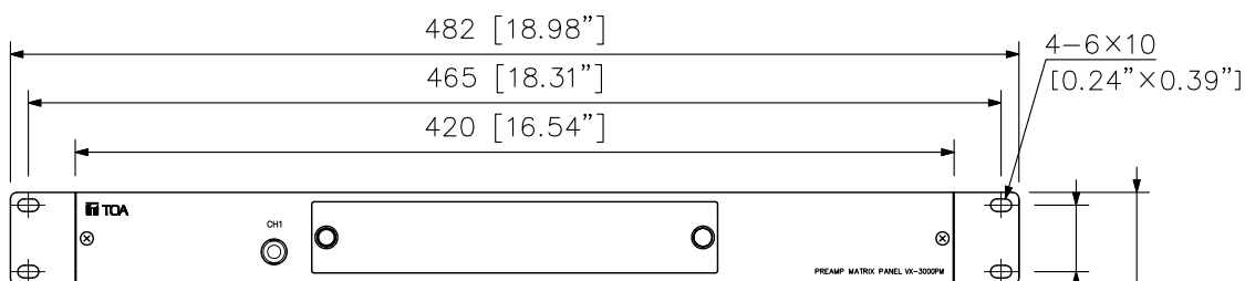
Front View
