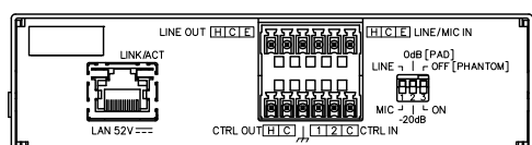
Rear View
