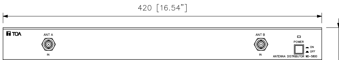
Front View
