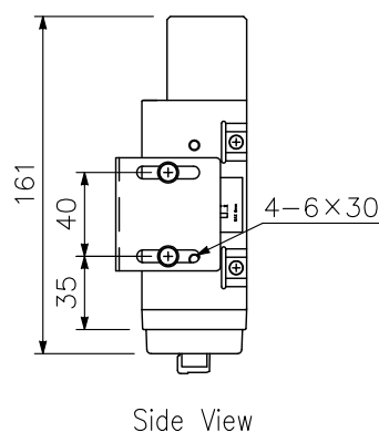
Accessory microphone (1/5)
