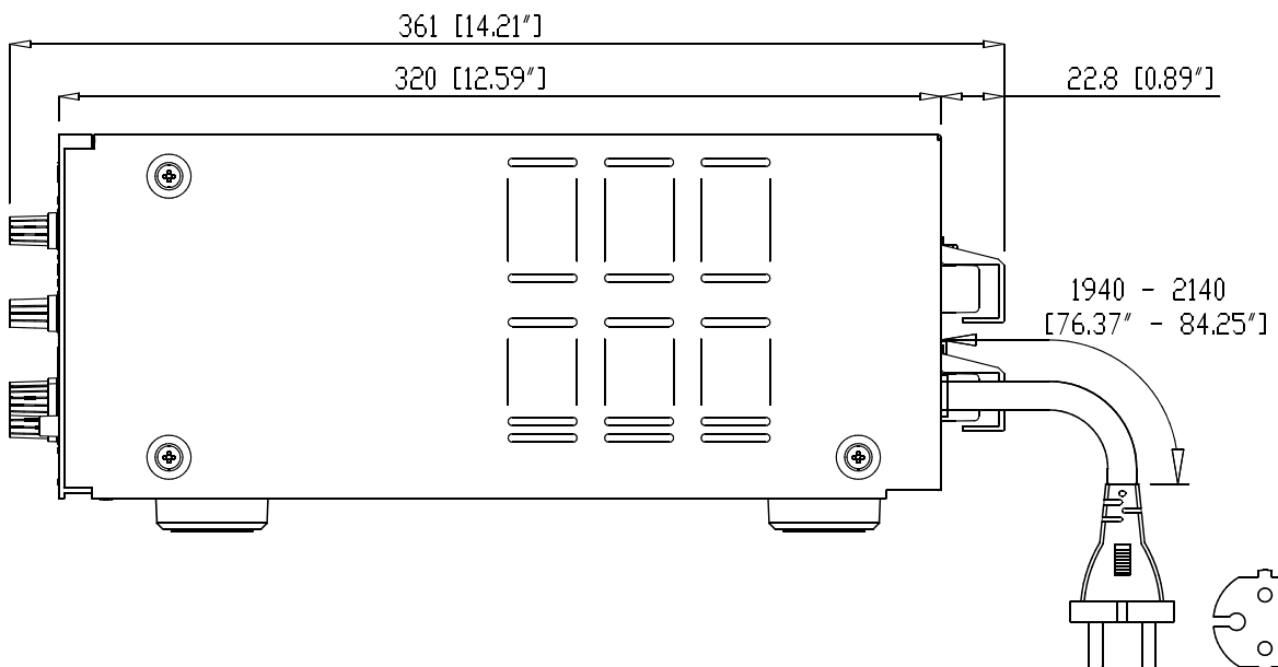
Right View
